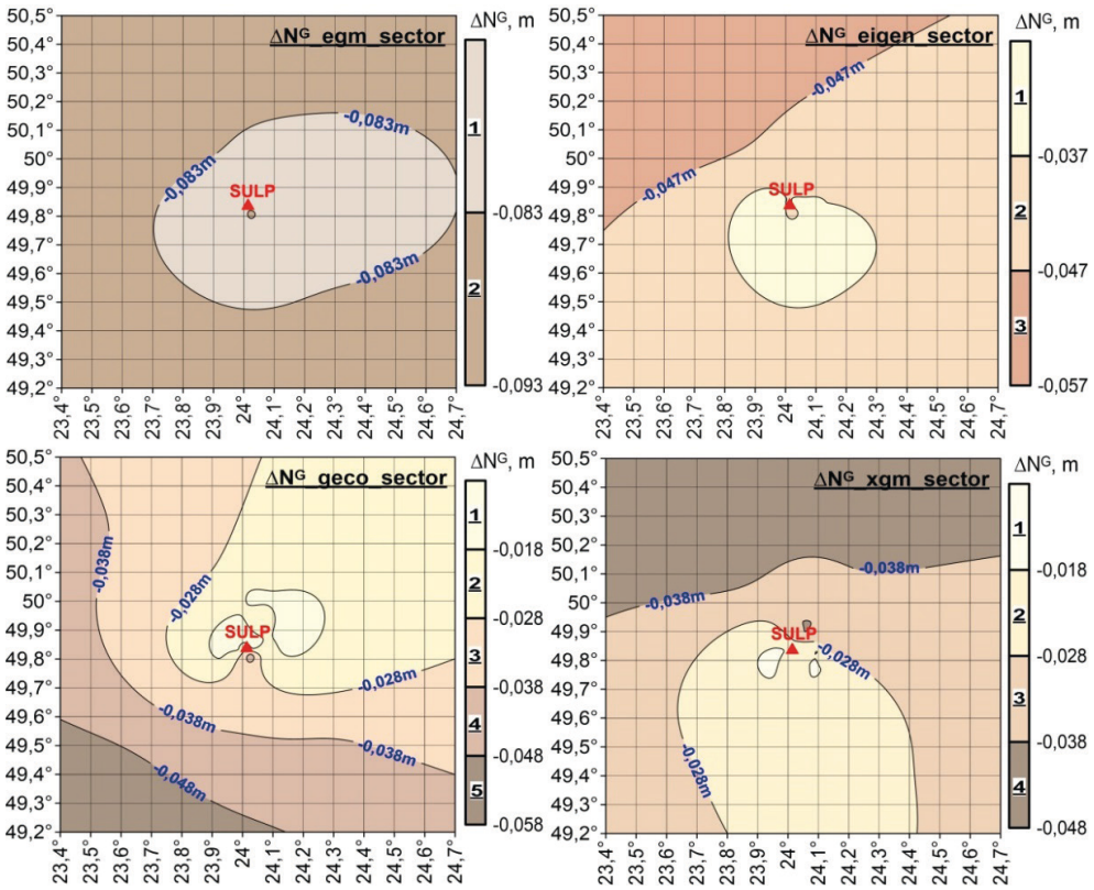
Fig. 5. Contour maps of averaged errors of geoid models EGM08, EIGEN-6C4, GECO and XGM2019e obtained by sector analysis
