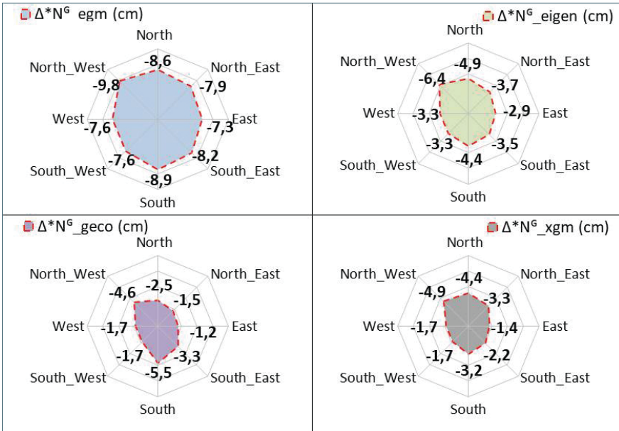
Fig. 4. Distribution of averaged errors of geoid models based on the results of sector analysis with respect to the permanent station SULP
