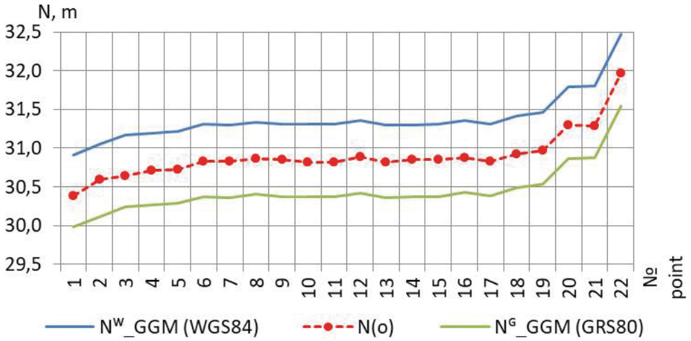
Fig. 2. Comparison heights of the calculated geoid and heights of the geoid model from the surface of the ellipsoid WGS84 and GRS80
