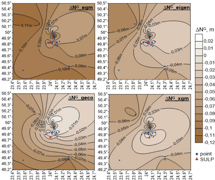
Fig. 3. Visualization of height errors of global geoid models based on the results of GNSS leveling
