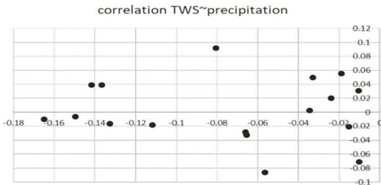
Fig. 8. Relation between TWS and precipitation, for the area of the Venezia Islands, unit: metres
